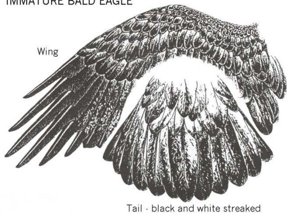
Spikes/Primaries Secondaries
